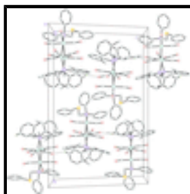
Fig. 2. The packing of the title compound, viewed down the a axis, showing the molecules linked into chains along c axis. Hydrogen atoms not involved in the hydrogen-bonding (dashed lines), minor disorder component and solvent molecules have been omitted for clarity.
