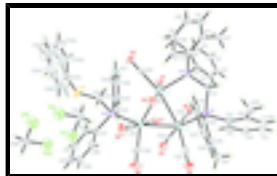
Fig. 1. The molecular structure of the title compound with 50% probability ellipsoids for non-H atoms. Minor disorder component is shown with open bonds. Atoms with suffix X are generated by the symmetry operation (-x, -y, 1 - z) .
